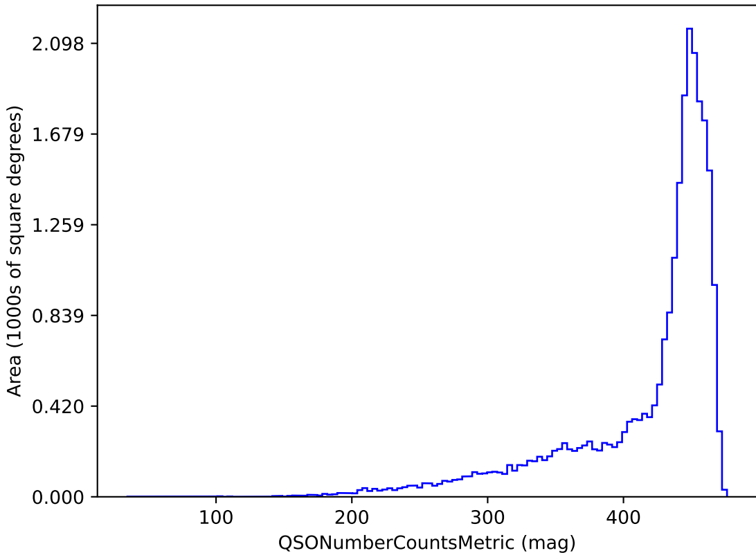
too_100_1v3.4_10yrs g band and non-DD: QSONumberCountsMetric
