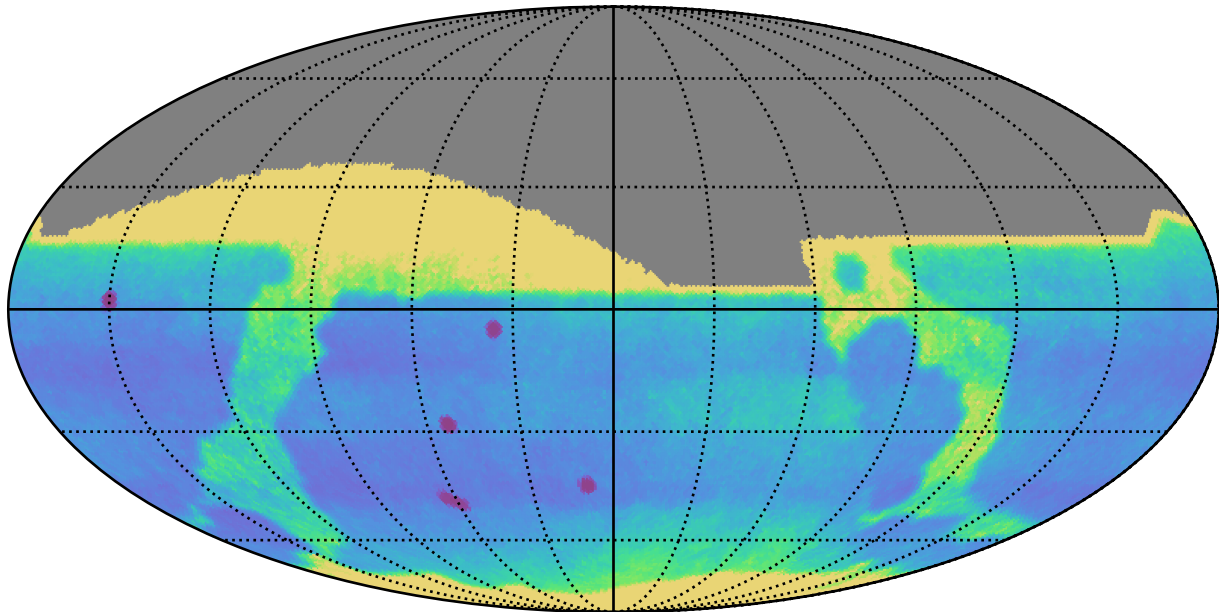
too_100_1v3.4_10yrs : Proper Motion Uncert @ 24.0
