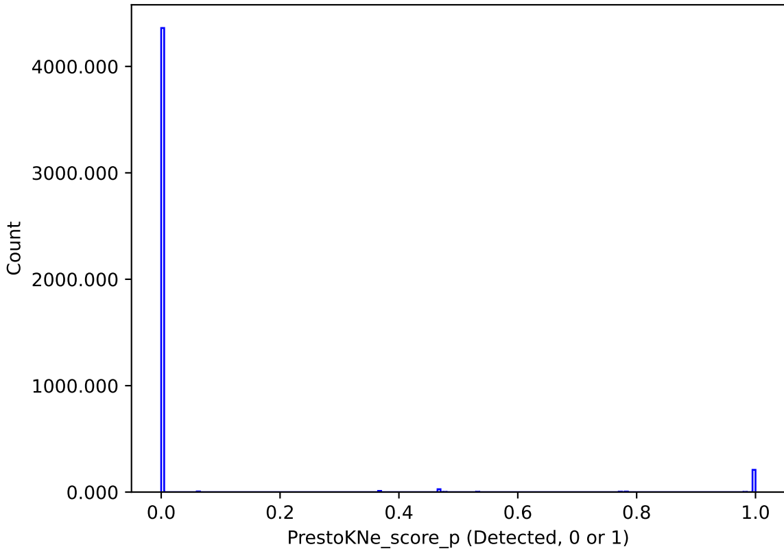
too_100_1v3.4_10yrs : PrestoKNe_score_p
