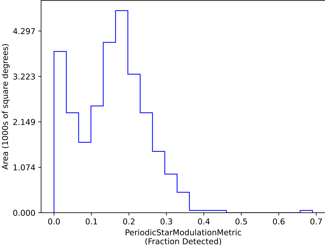
too_100_1v3.4_10yrs dm 20 interval 30 RRC Year 1-2: PeriodicStarModulationMetric
