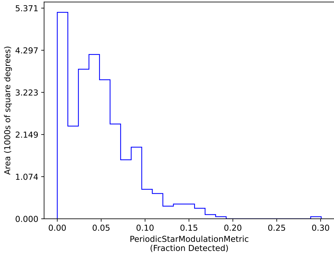
too_100_1v3.4_10yrs dm 20 interval 15 RRc Year 1-2: PeriodicStarModulationMetric
