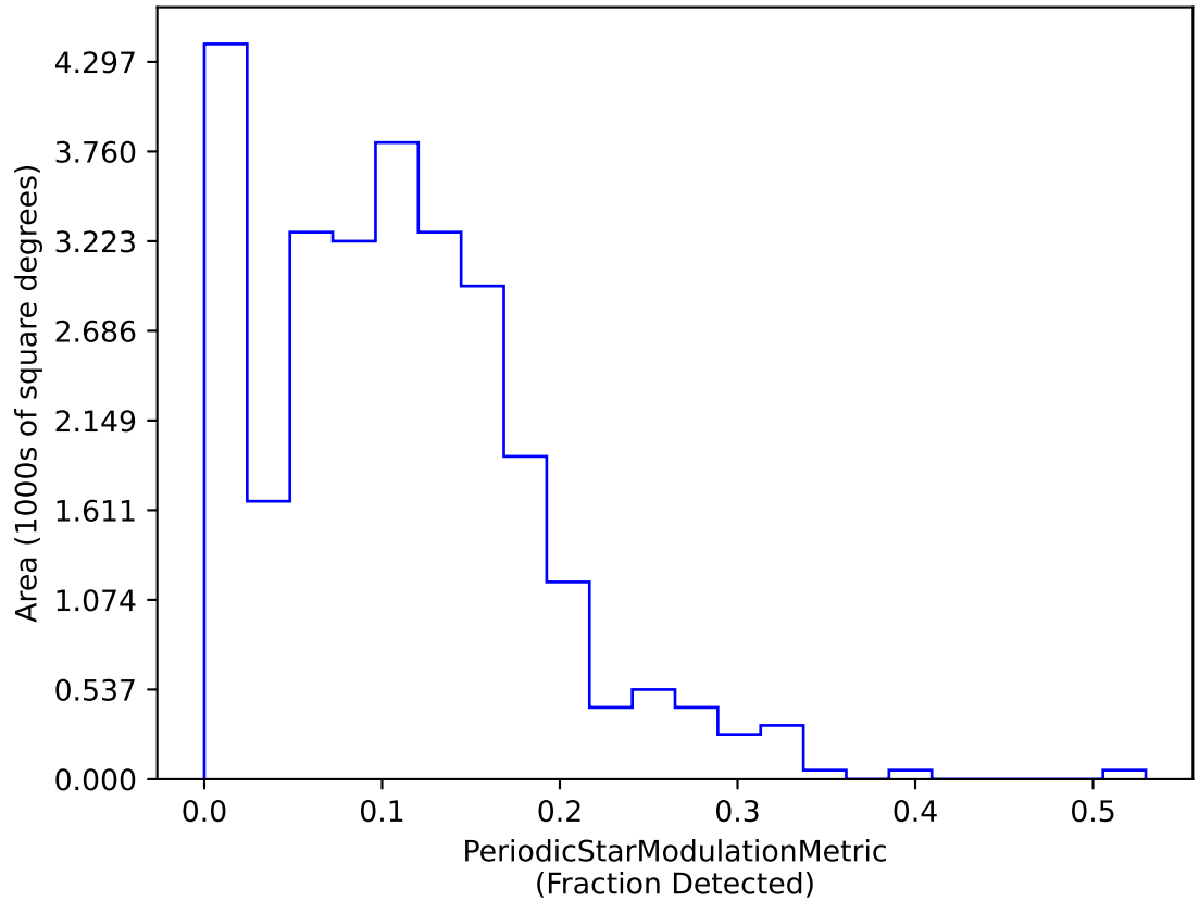
too_100_1v3.4_10yrs dm 19 interval 15 RRc Year 1-2: PeriodicStarModulationMetric
