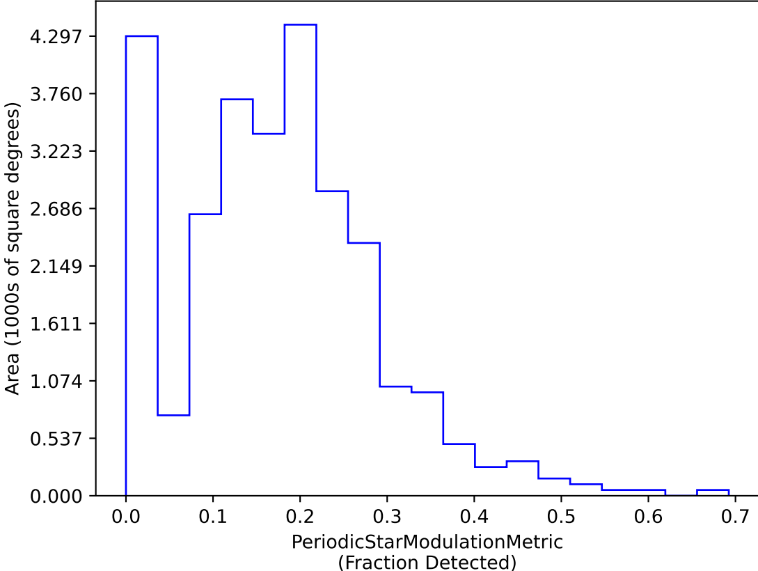
too_100_1v3.4_10yrs dm 18 interval 15 RRC Year 1-2: PeriodicStarModulationMetric
