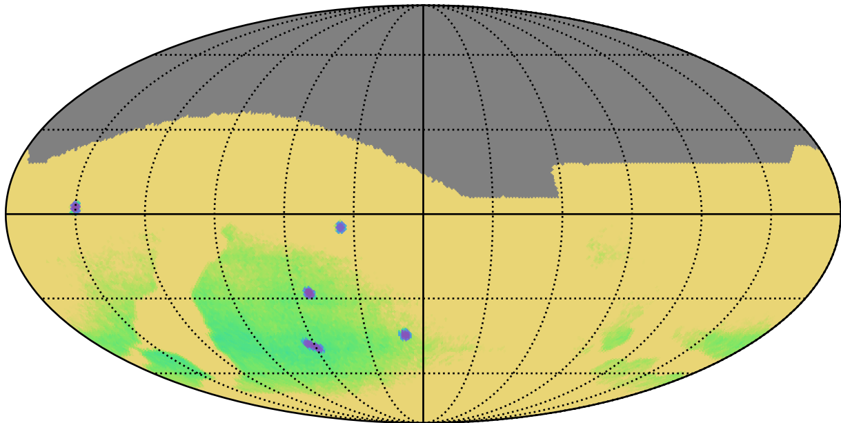
too_100_1v3.4_10yrs : Parallax Uncert @ 22.4
