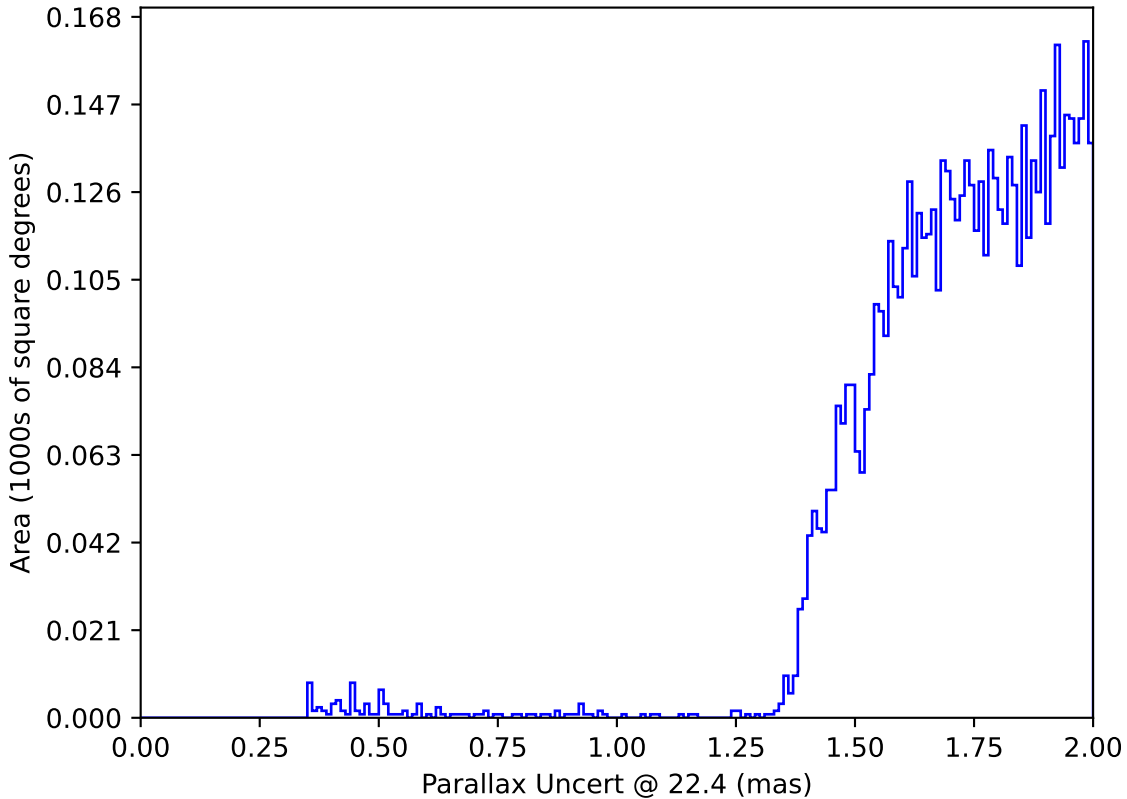
too_100_1v3.4_10yrs : Parallax Uncert @ 22.4
