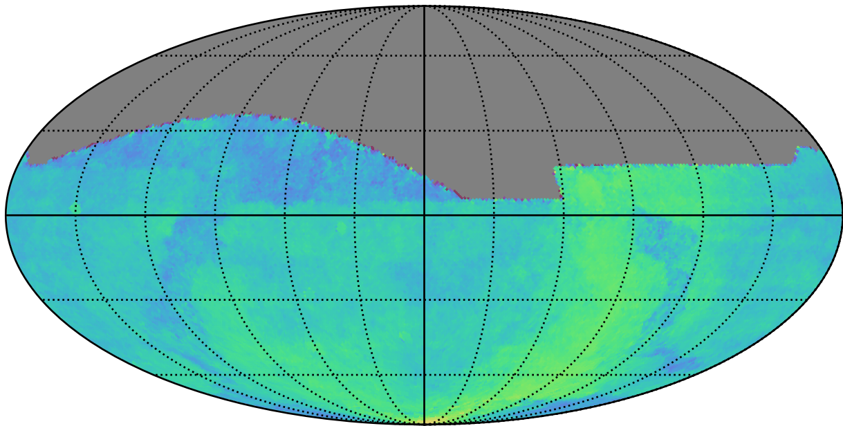
too_100_1v3.4_10yrs : Parallax Coverage @ 24.0
