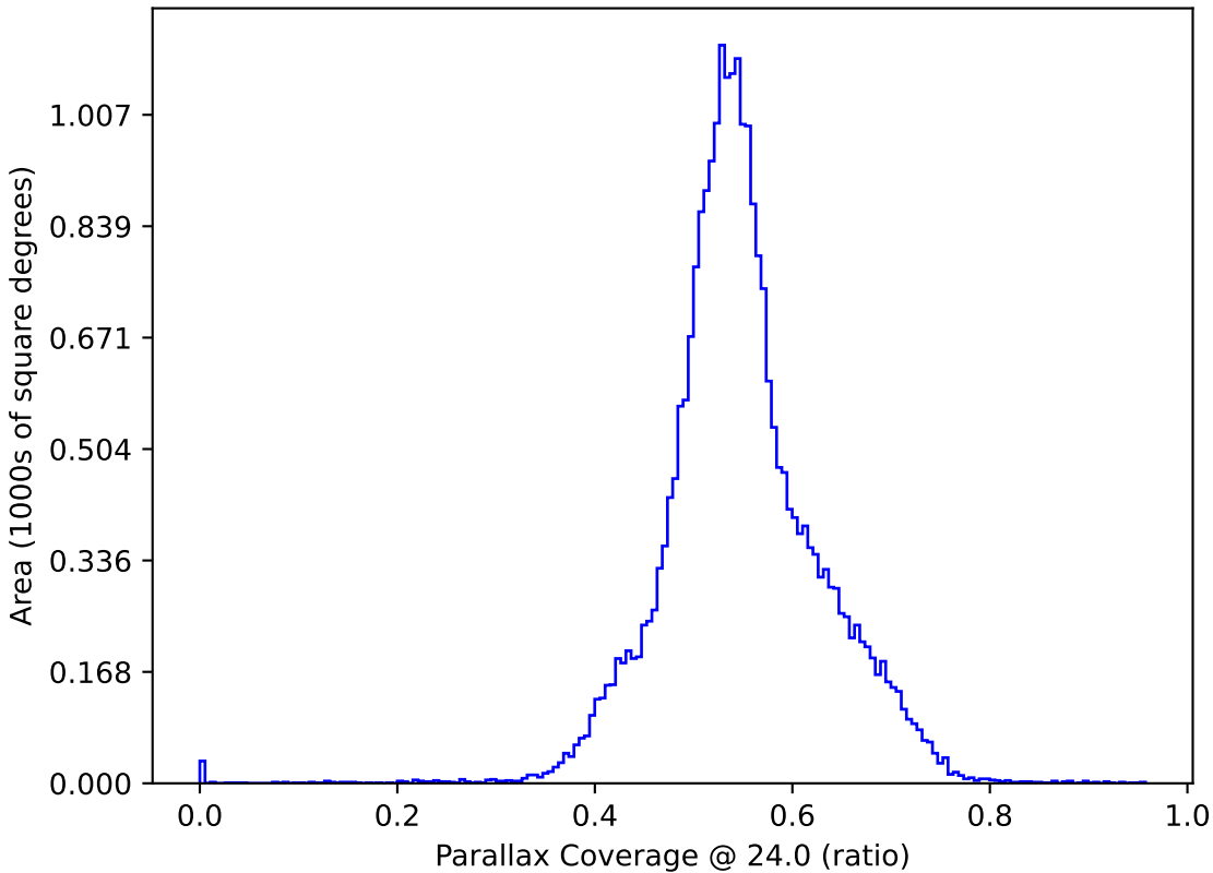
too_100_1v3.4_10yrs : Parallax Coverage @ 24.0
