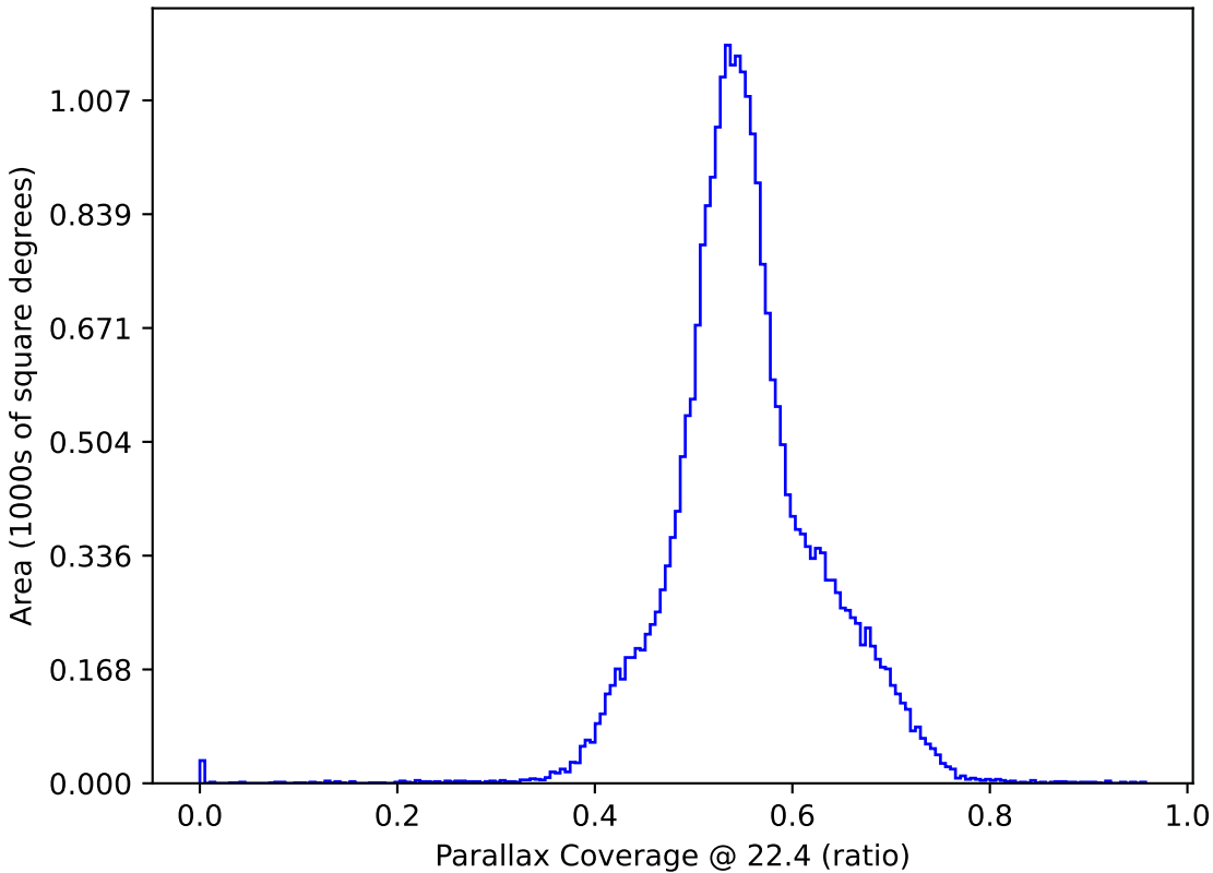
too_100_1v3.4_10yrs : Parallax Coverage @ 22.4
