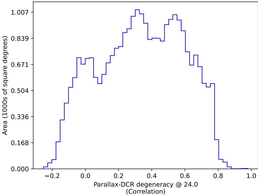
too_100_1v3.4_10yrs : Parallax-DCR degeneracy @ 24.0
