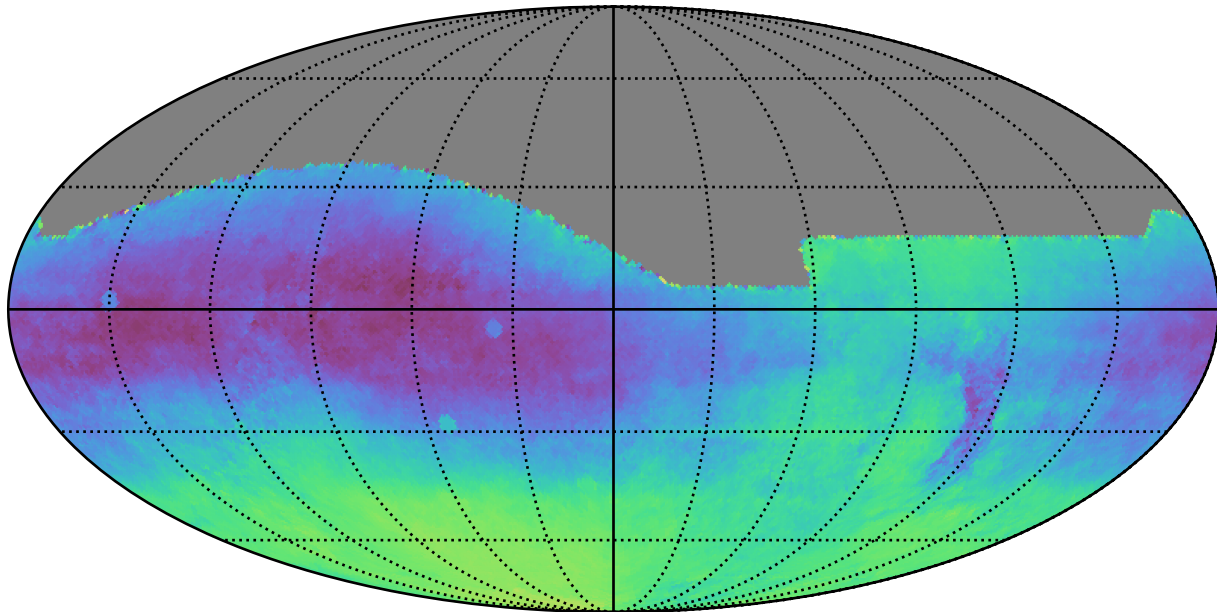
too_100_1v3.4_10yrs : Parallax-DCR degeneracy @ 22.4
