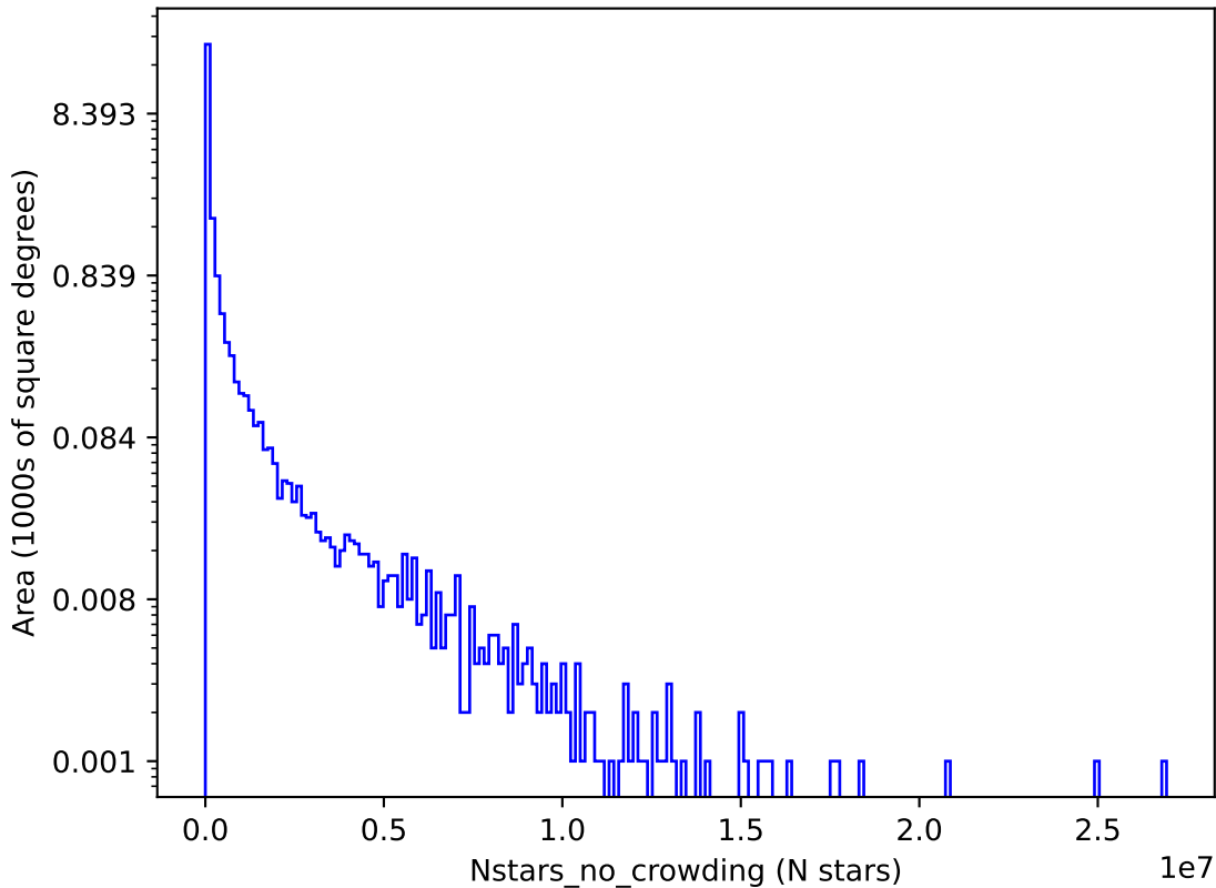
too_100_1v3.4_10yrs z: Nstars_no_crowding
