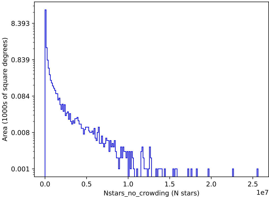
too_100_1v3.4_10yrs y: Nstars_no_crowding
