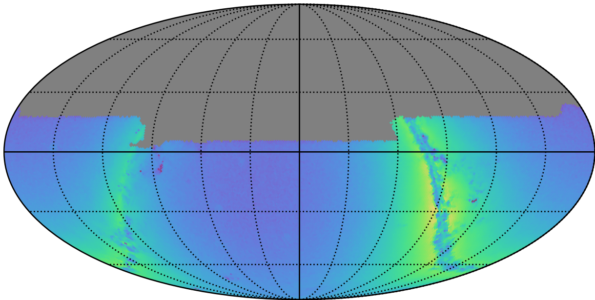
too_100_1v3.4_10yrs u: Nstars_no_crowding
