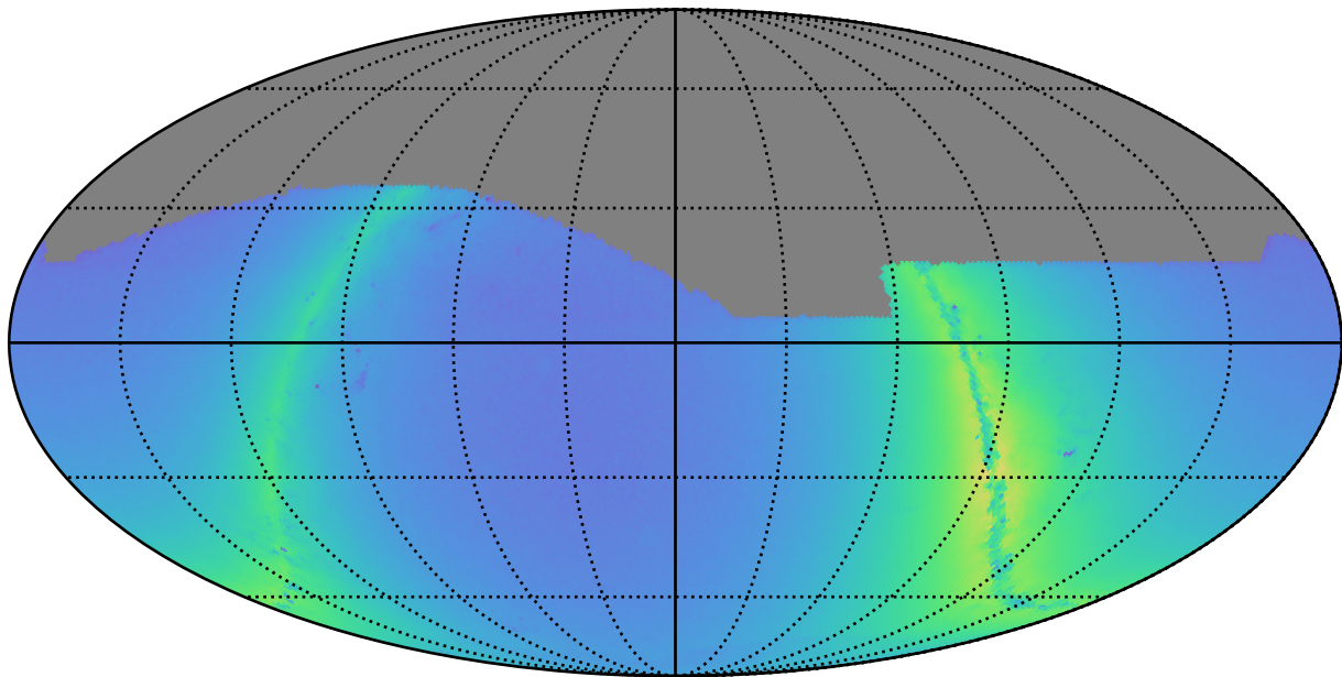
too_100_1v3.4_10yrs r: Nstars_no_crowding
