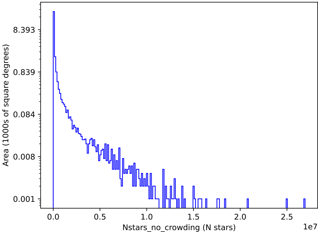
too_100_1v3.4_10yrs i: Nstars_no_crowding
