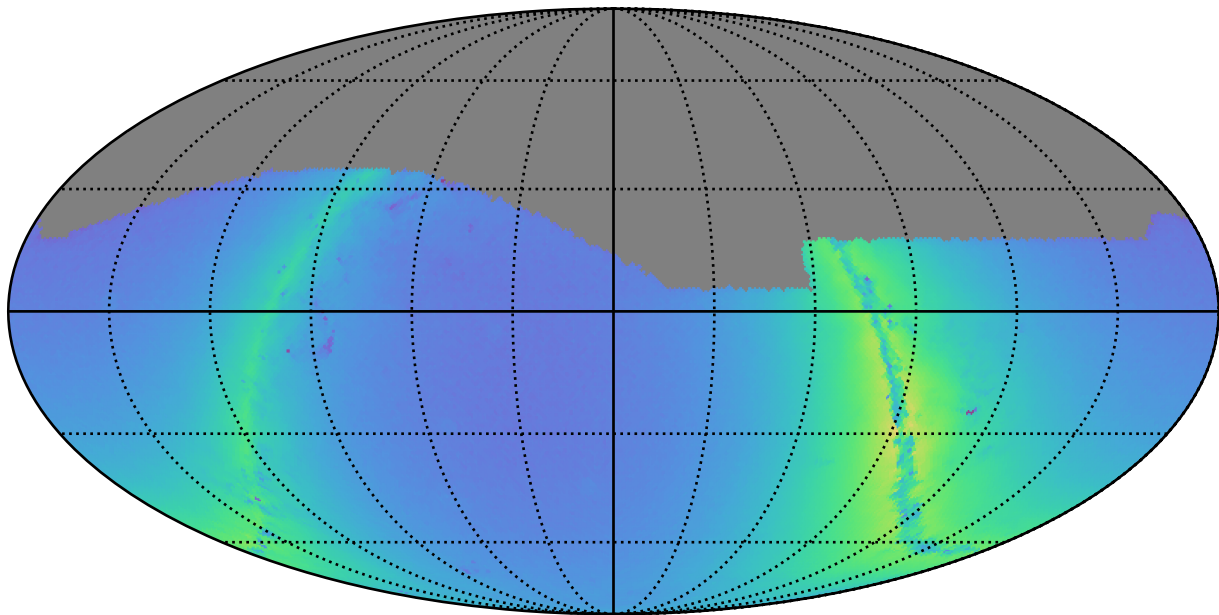
too_100_1v3.4_10yrs g: Nstars_no_crowding
