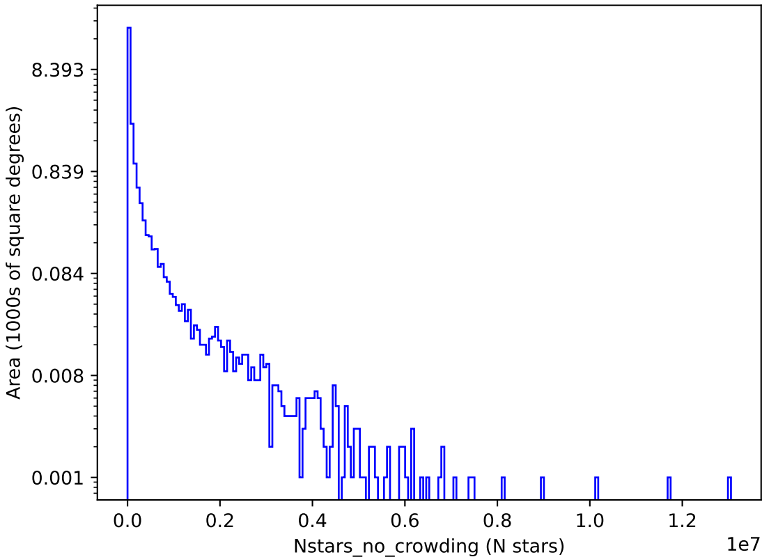
too_100_1v3.4_10yrs g: Nstars_no_crowding
