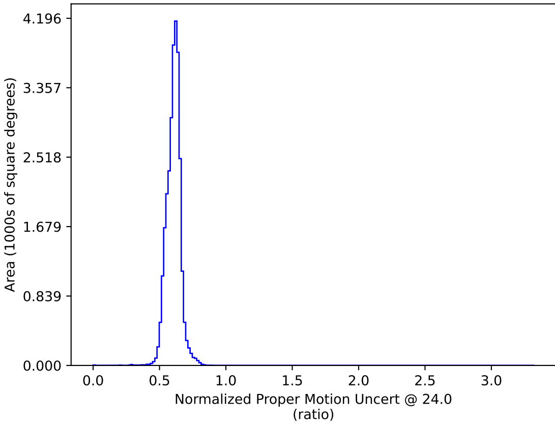
too_100_1v3.4_10yrs : Normalized Proper Motion Uncert @ 24.0
