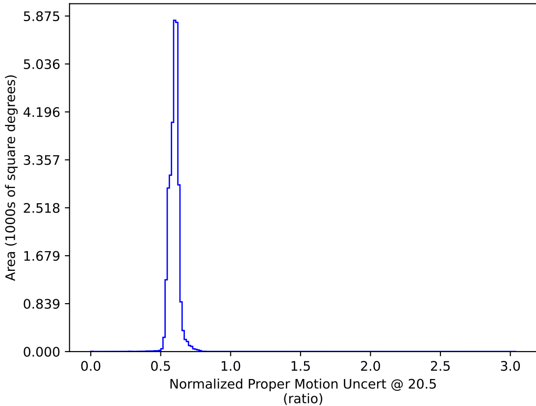
too_100_1v3.4_10yrs : Normalized Proper Motion Uncert @ 20.5
