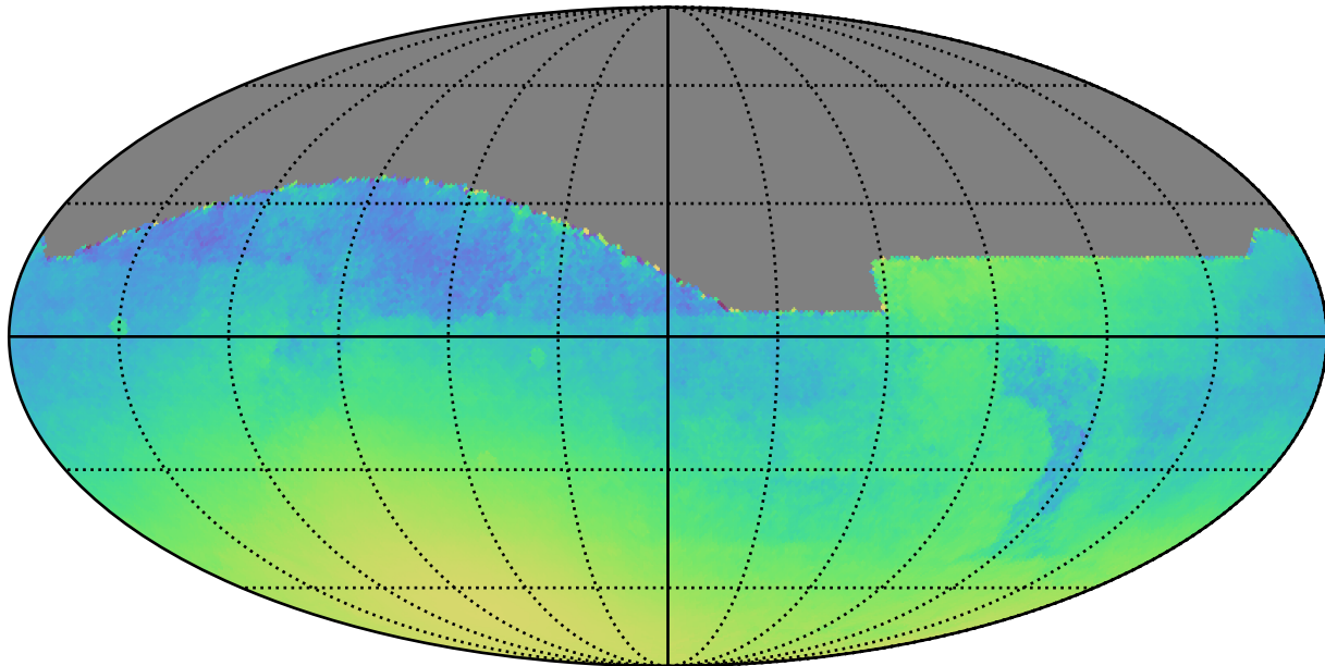
too_100_1v3.4_10yrs : Normalized Parallax Uncert @ 24.0
