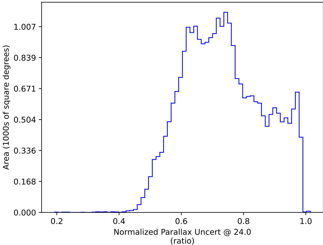
too_100_1v3.4_10yrs : Normalized Parallax Uncert @ 24.0
