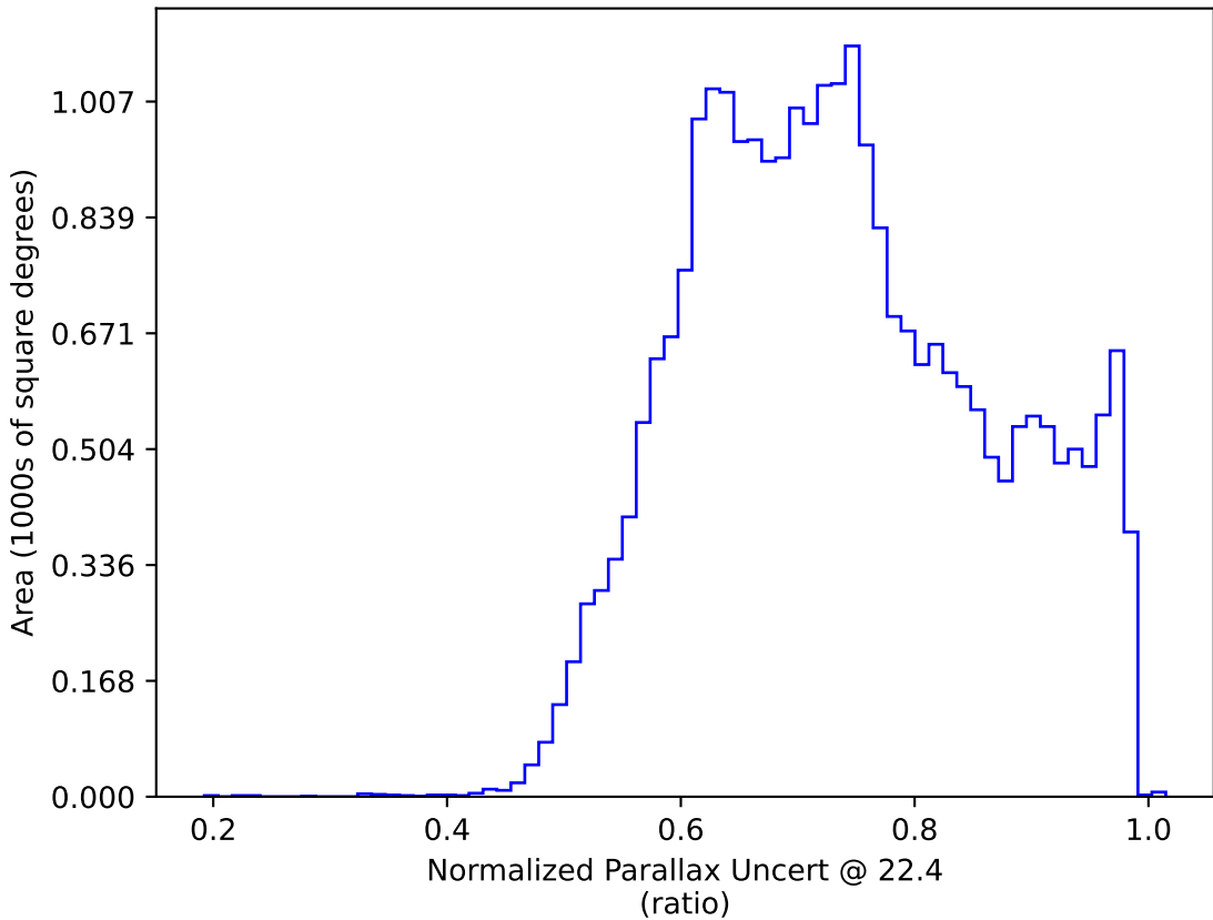
too_100_1v3.4_10yrs : Normalized Parallax Uncert @ 22.4
