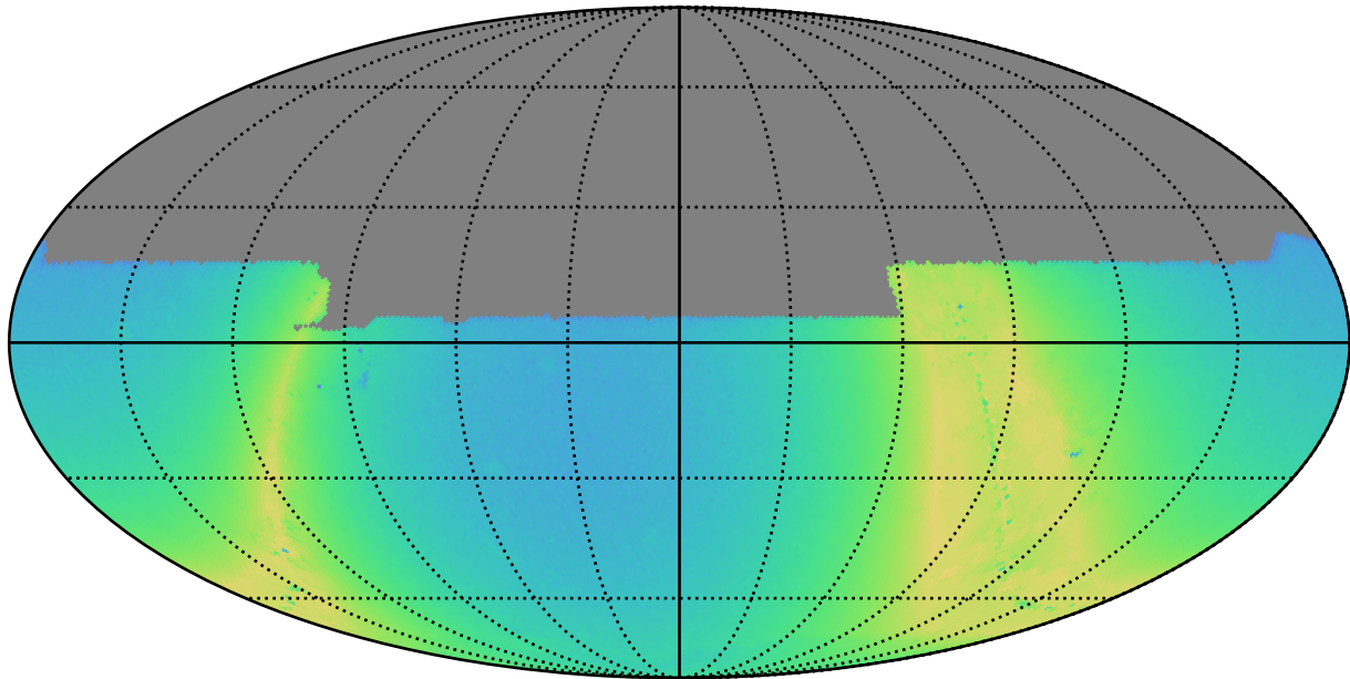
too_100_1v3.4_10yrs y: N stars to Precision 0.20
