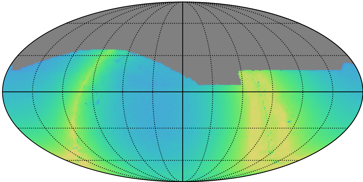
too_100_1v3.4_10yrs r: N stars to Precision 0.20
