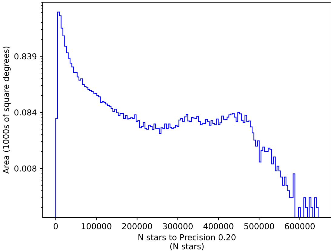
too_100_1v3.4_10yrs r: N stars to Precision 0.20
