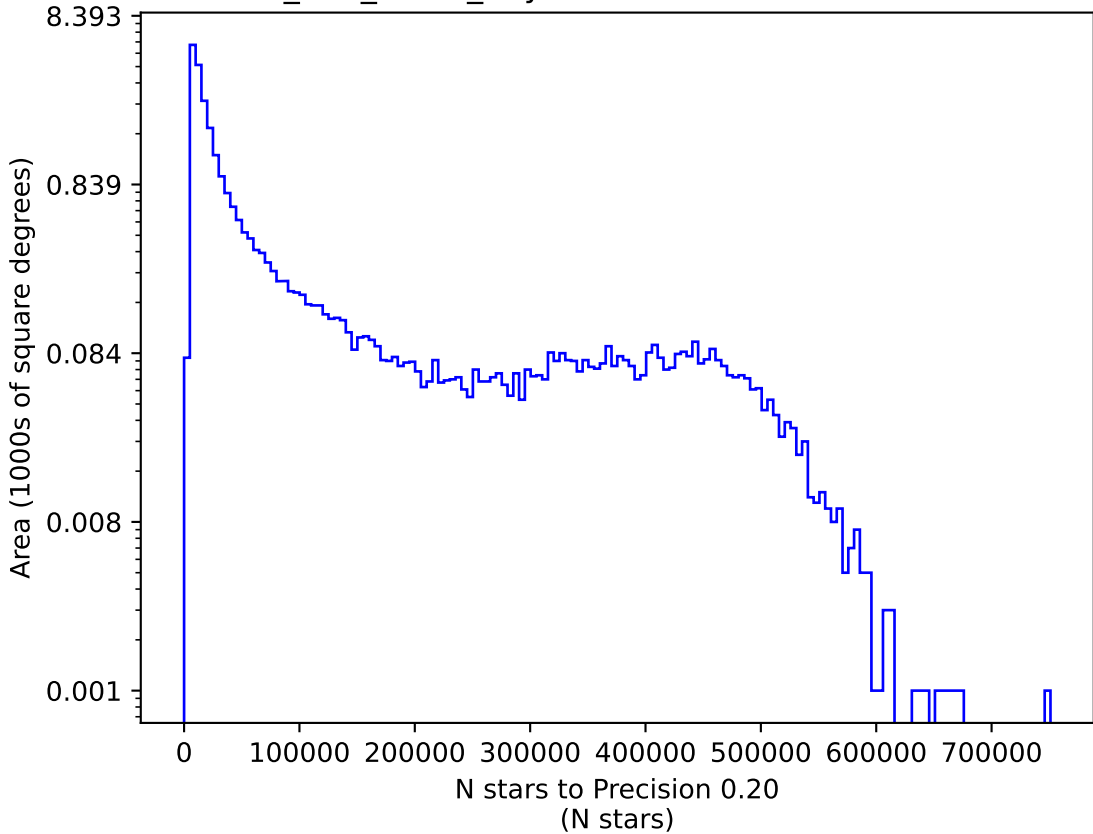
too_100_1v3.4_10yrs i: N stars to Precision 0.20
