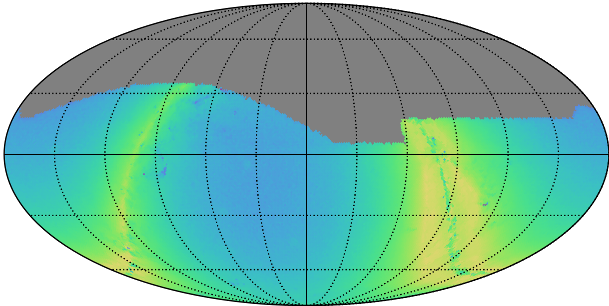
too_100_1v3.4_10yrs g: N stars to Precision 0.20
