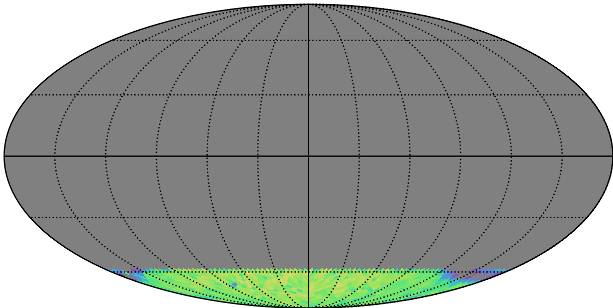
too_100_1v3.4_10yrs gi SCP: LVDwarfs
