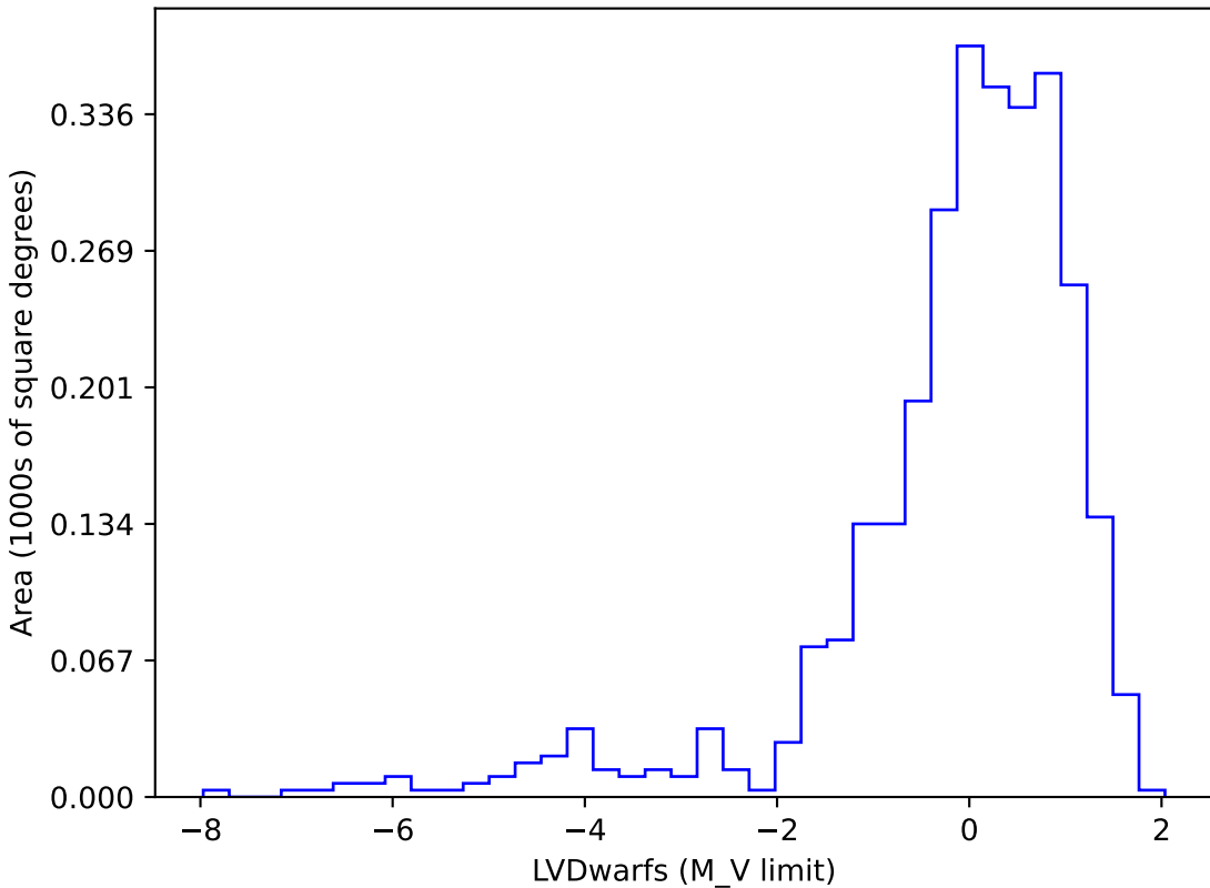
too_100_1v3.4_10yrs gi SCP: LVDwarfs
