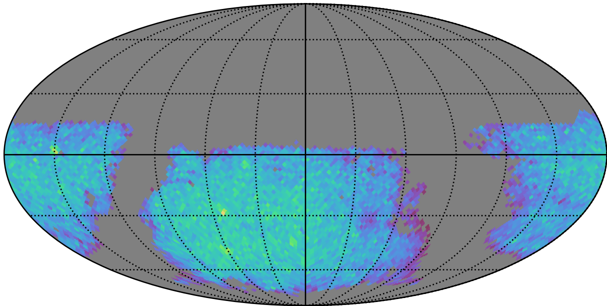
too_100_1v3.4_10yrs gi: LVDwarfs
