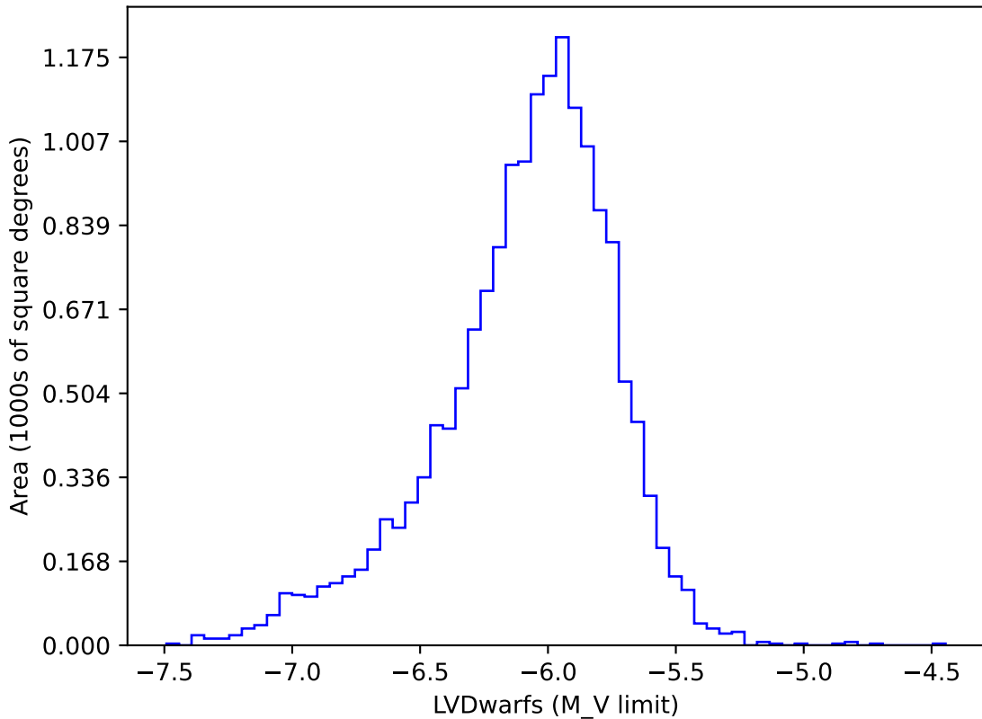
too_100_1v3.4_10yrs gi: LVDwarfs
