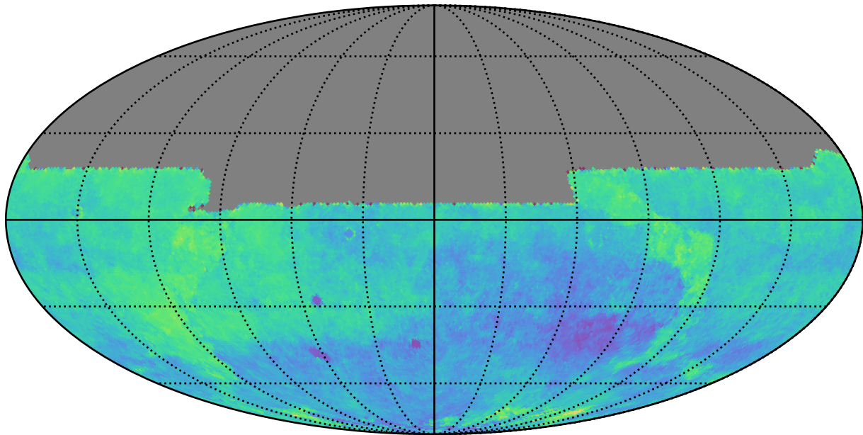
too_100_1v3.4_10yrs y: Kuiper rotSkyPos
