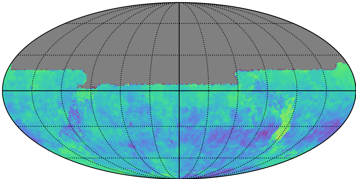
too_100_1v3.4_10yrs u: Kuiper rotSkyPos
