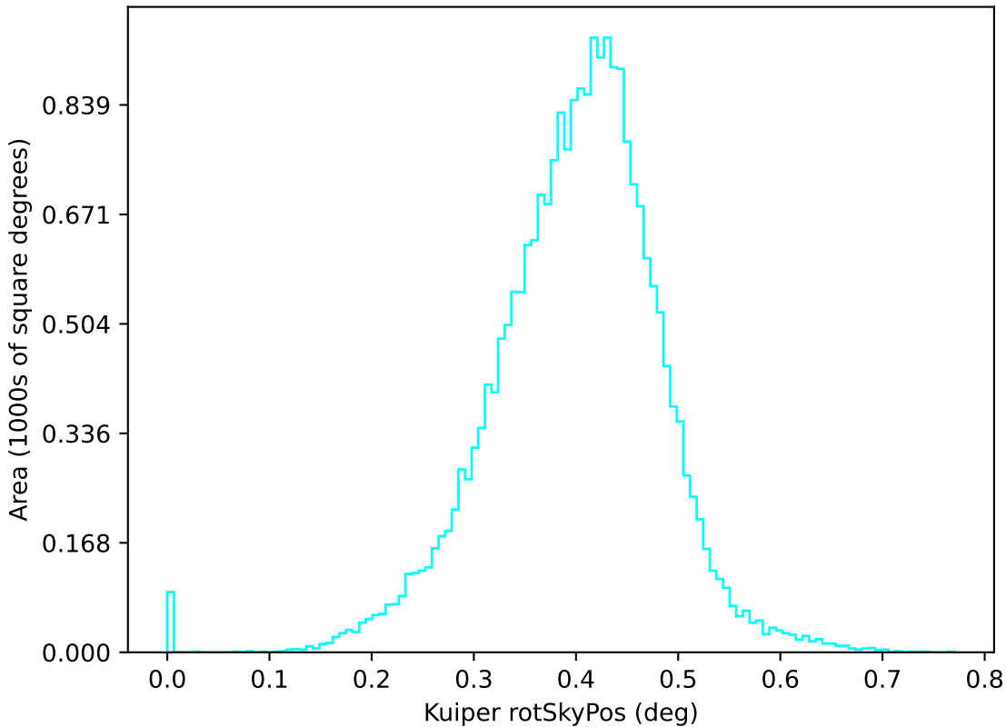
too_100_1v3.4_10yrs u: Kuiper rotSkyPos
