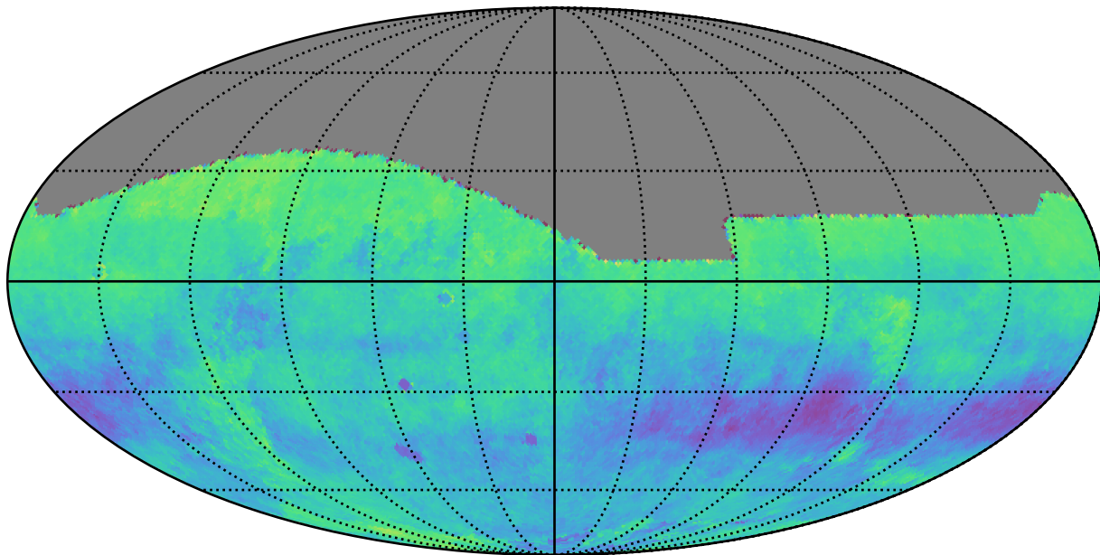
too_100_1v3.4_10yrs r: Kuiper rotSkyPos
