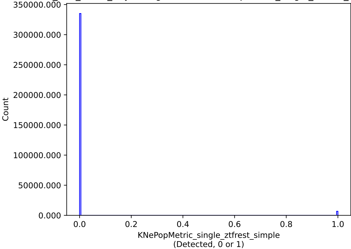
too_100_1v3.4_10yrs single model: KNePopMetric_single_ztfrest_simple
