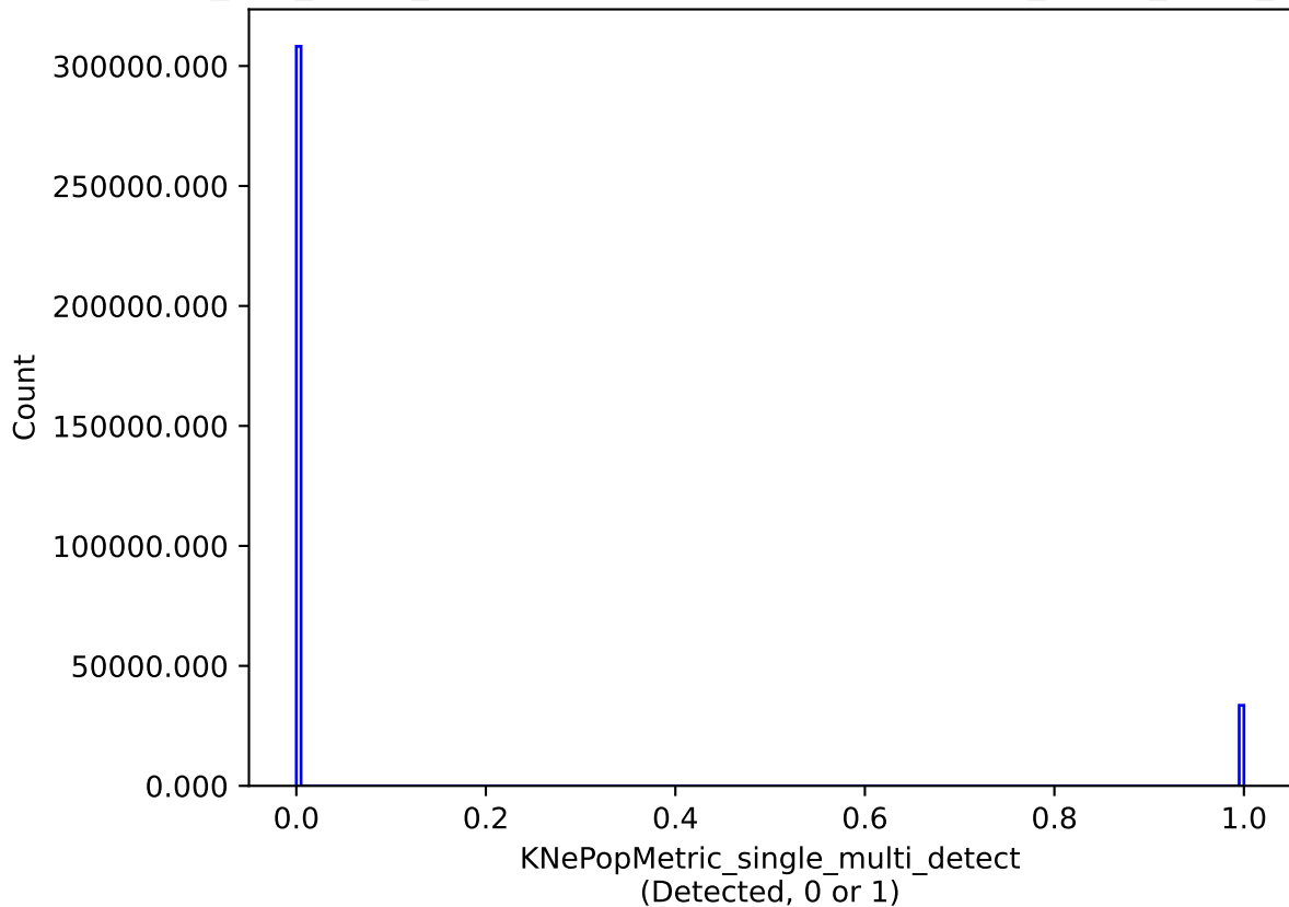
too_100_1v3.4_10yrs single model: KNePopMetric_single_multi_detect
