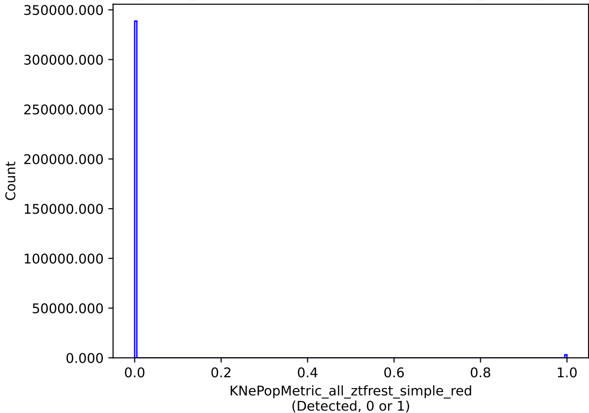
too_100_1v3.4_10yrs all models: KNePopMetric_all_ztfrest_simple_red
