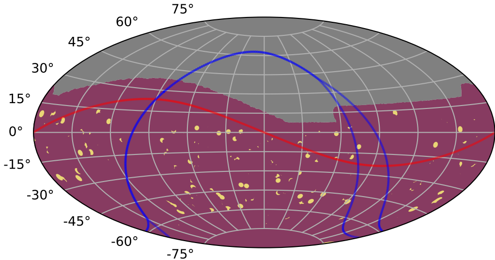
too_100_1v3.4_10yrs all models: KNePopMetric_all_ztfrest_simple
