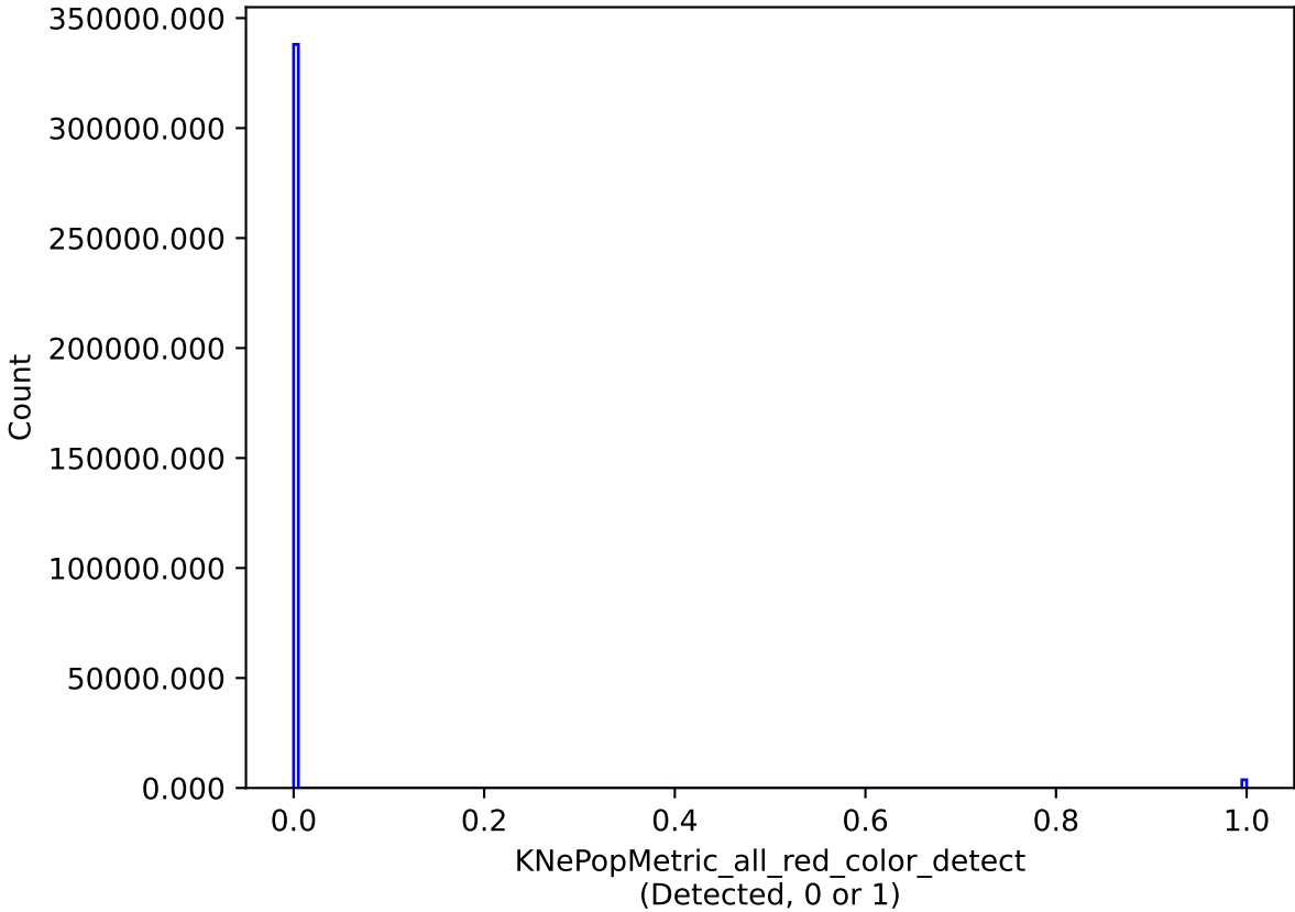
too_100_1v3.4_10yrs all models: KNePopMetric_all_red_color_detect
