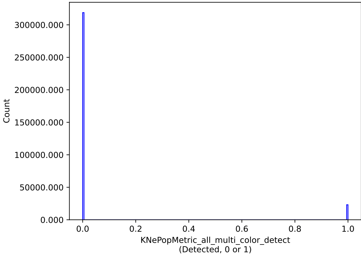
too_100_1v3.4_10yrs all models: KNePopMetric_all_multi_color_detect
