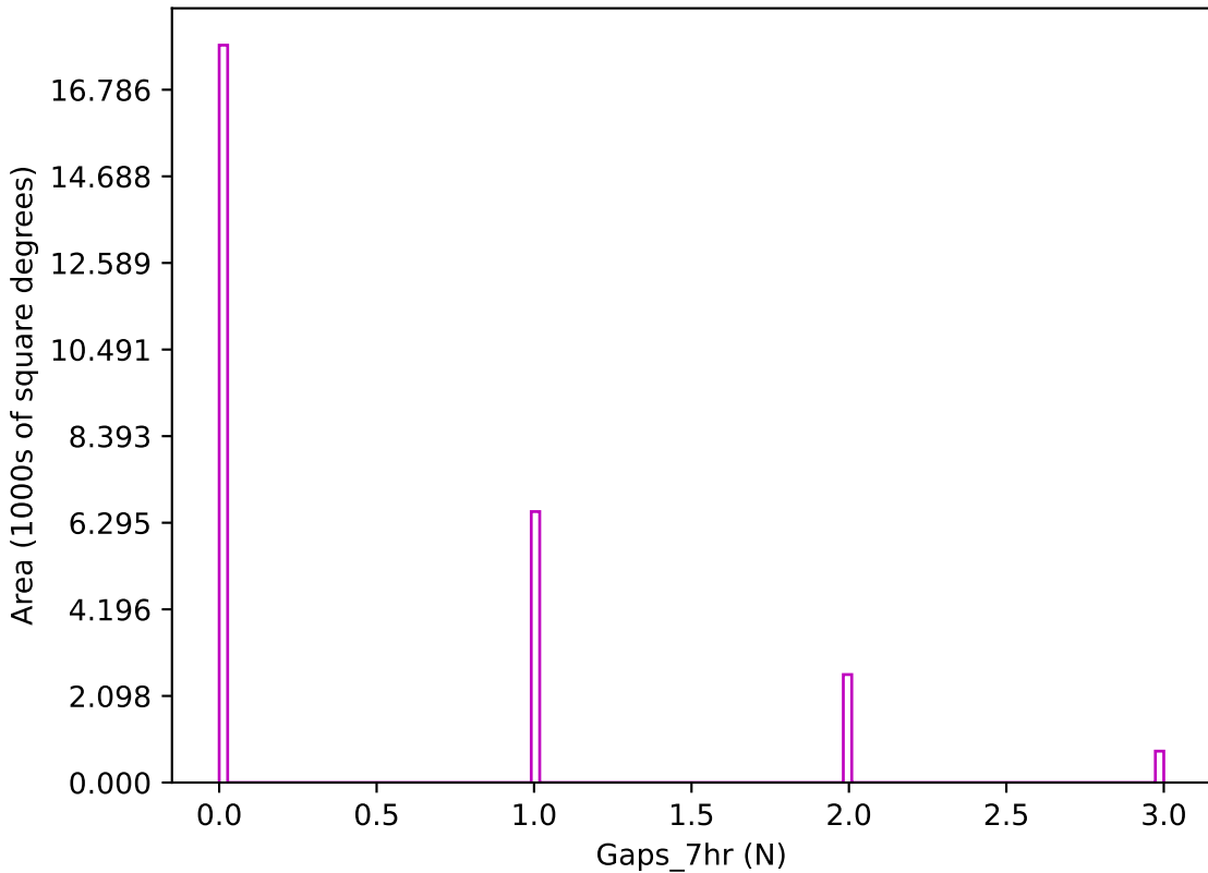
too_100_1v3.4_10yrs z band: Gaps_7hr
