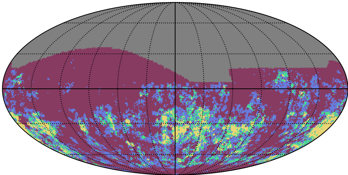
too_100_1v3.4_10yrs i band: Gaps_7hr
