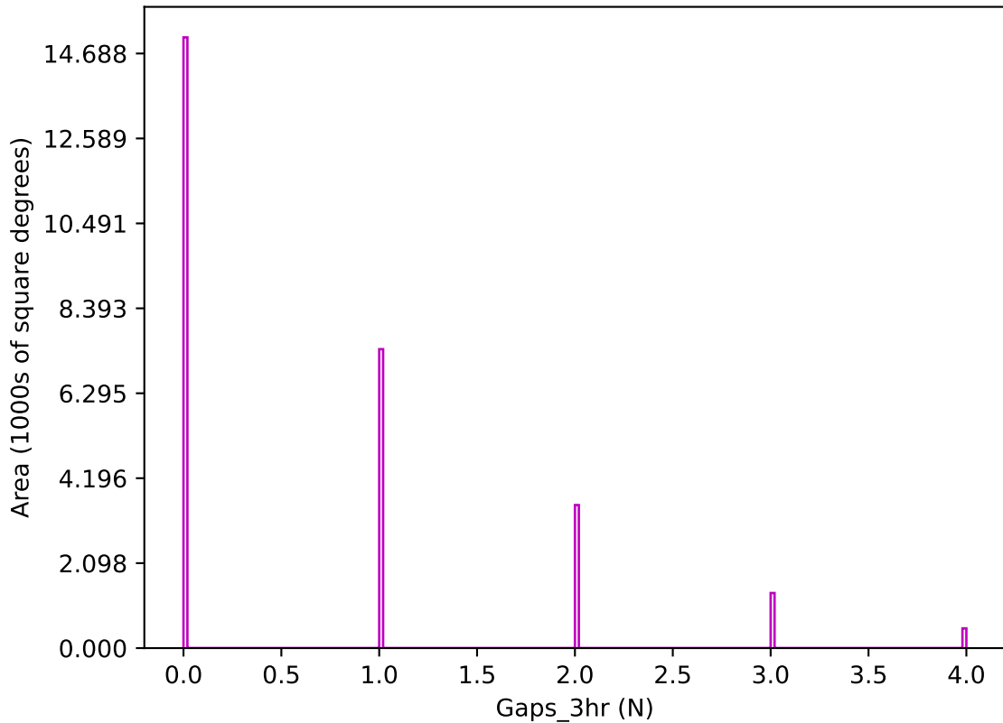
too_100_1v3.4_10yrs z band: Gaps_3hr
