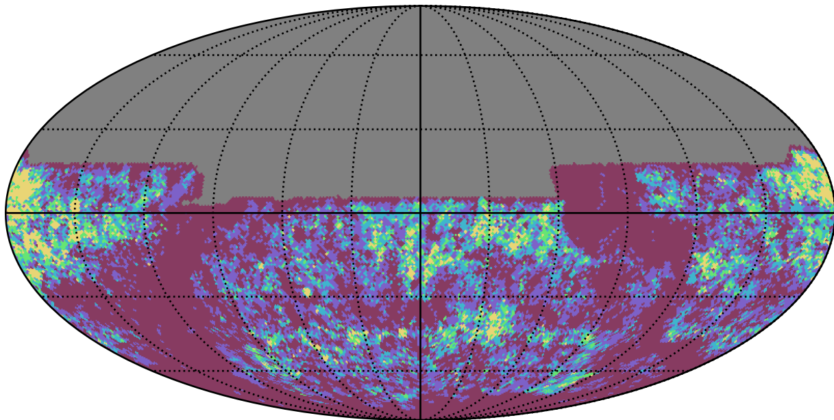
too_100_1v3.4_10yrs y band: Gaps_3hr
