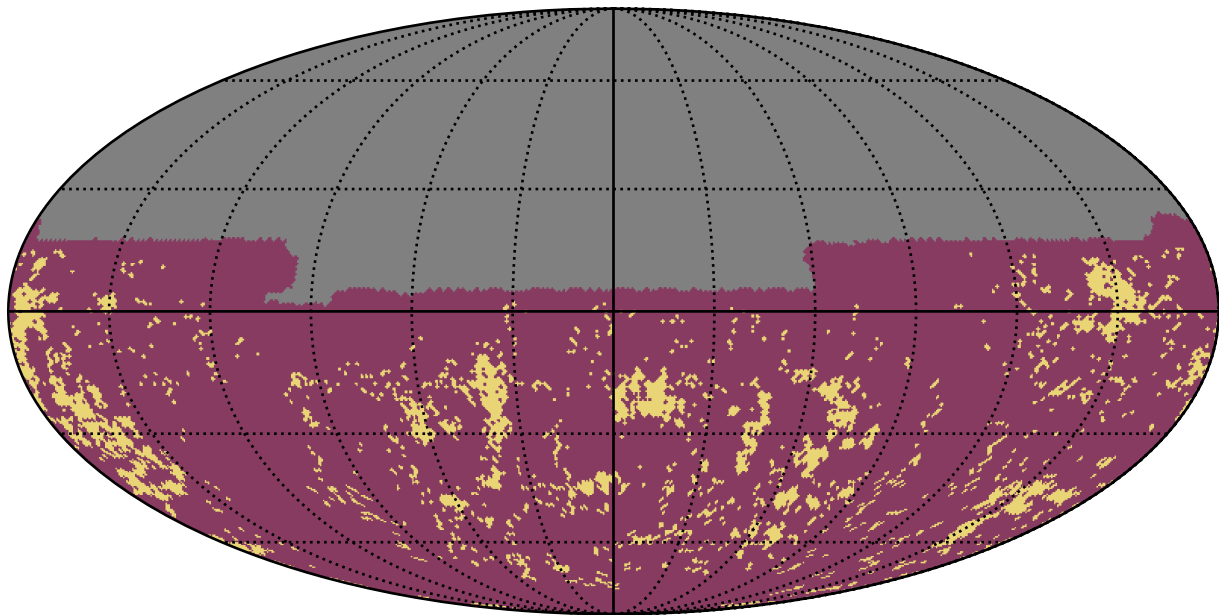
too_100_1v3.4_10yrs u band: Gaps_3hr
